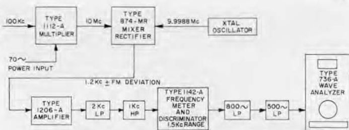
Figure 10. Block diagram of system used for the measurement of fm noise level of the Type 1112-A Standard-Frequency Multiplier.
