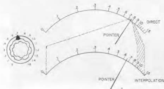
Figure 2. Illustrating meter scale-expansion. With METER FUNCTION switch set on DIRECT, meter indicates 0.77, as shown at top. When set on INTERPOLATION, as shown at bottom, the frequency meter indicates 0.766. The first digit (.7) is set on the INTERPOLATION OFFSET FREQUENCY switch and the interval from .7 to .8 is expanded to cover the scale from 0 to 1.0, so that the second and third digits (.66) are easily read on the meter.
