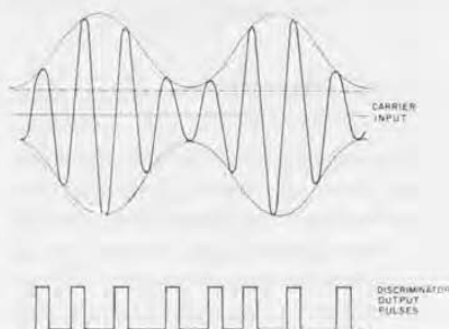
Figure 8. Illustrating the apparent frequency modulation produced by an amplitude-modulated wave.
