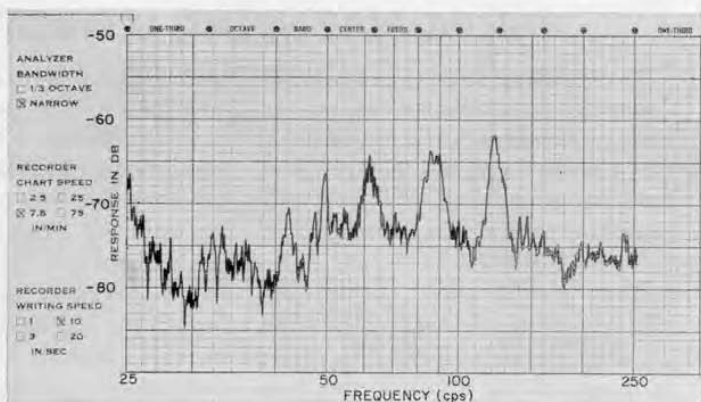
Figure 12. Automatic plot of flutter in an audio tape recorder, made with the equipment shown in Figure 11. A response of -60 db corresponds to a frequency deviation of 0.1% of the test frequency.
