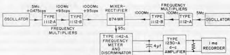
Figure 6. Arrangement of equipment used to measure the relative drift of two 5-Mc oscillators. The 5-Mc frequencies were multiplied up to 1000 Mc to magnify their frequency drift.
